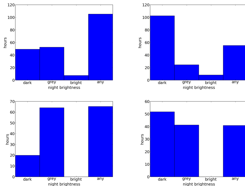
Figure 2: In the upper left panel, the amount of hours requested in the different types of night brightness in semester 2016B (the peak for “any” type of night is mostly due to ToO and variability monitoring programs). In the upper right panel, the same plot for semester 2017A. Semesters 2017B and 2018A are shown in the lower left and lower right panel respectively.
