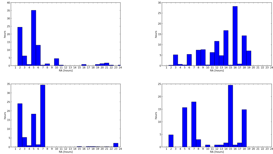
Figure 3: The time requested distributed in the different intervals of right ascension for periods, from top to bottom and left to right, 2016B, 2017A, 2017B and 2018A. Note that, for obvious reasons, ToO programs are not included in this plot.
